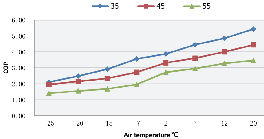
CGK030V3L/CGK-030V3L COP
