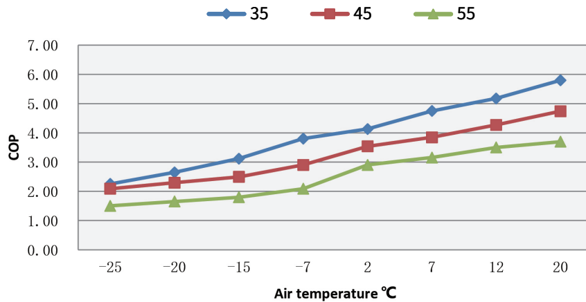
CGK050V3L/CGK-050V3L COP
