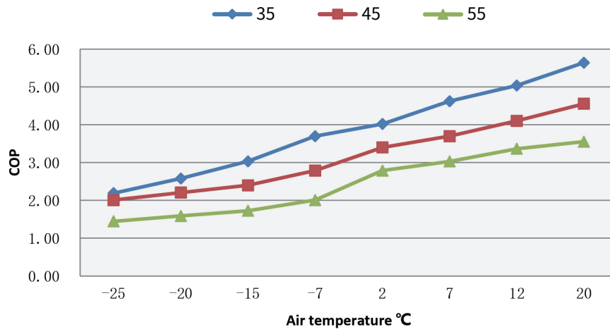
CGK060V3L/CGK-060V3L COP
